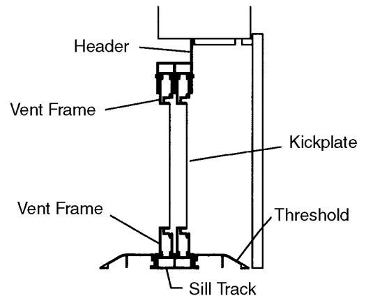
Regular Mount Side View
