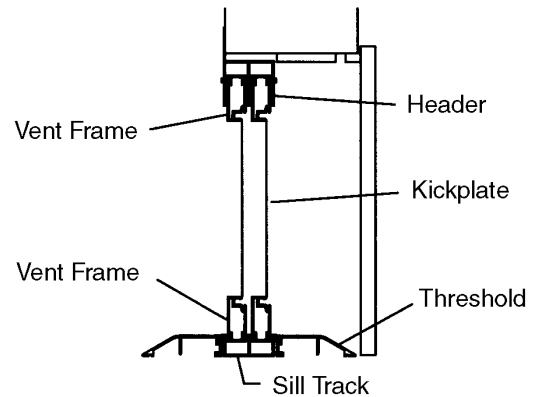
Reverse Mount Side View
