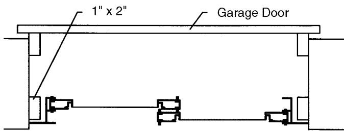
Reverse Mount Top View
