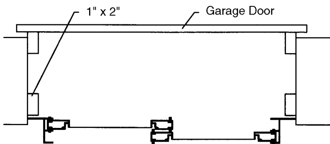
Regular Mount Top View
